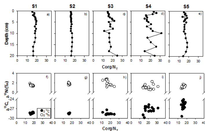
Figure 3: Ratios of C_{\text{org}}/N_T with depth, \delta^{13}\text{C}:C_{\text{org}}/N_T and \delta^{15}\text{N}:C_{\text{org}}/N_T in the sediments collected in September 2012 at sites S1-S5 in the Ciénega Tamasopo wetland (San Luis Potosi, Mexico).
