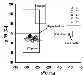
Figure 4: Stable Isotope values \delta^{15}\text{N} vs \delta^{13}\text{C} for samples from Ciénega Tamasopo at sites S1- S5, C3 and C4 plants, phytoplankton and sewage. Value ranges of \delta^{15}\text{N} vs \delta^{13}\text{C} from the literature are shown by the boxed areas.
