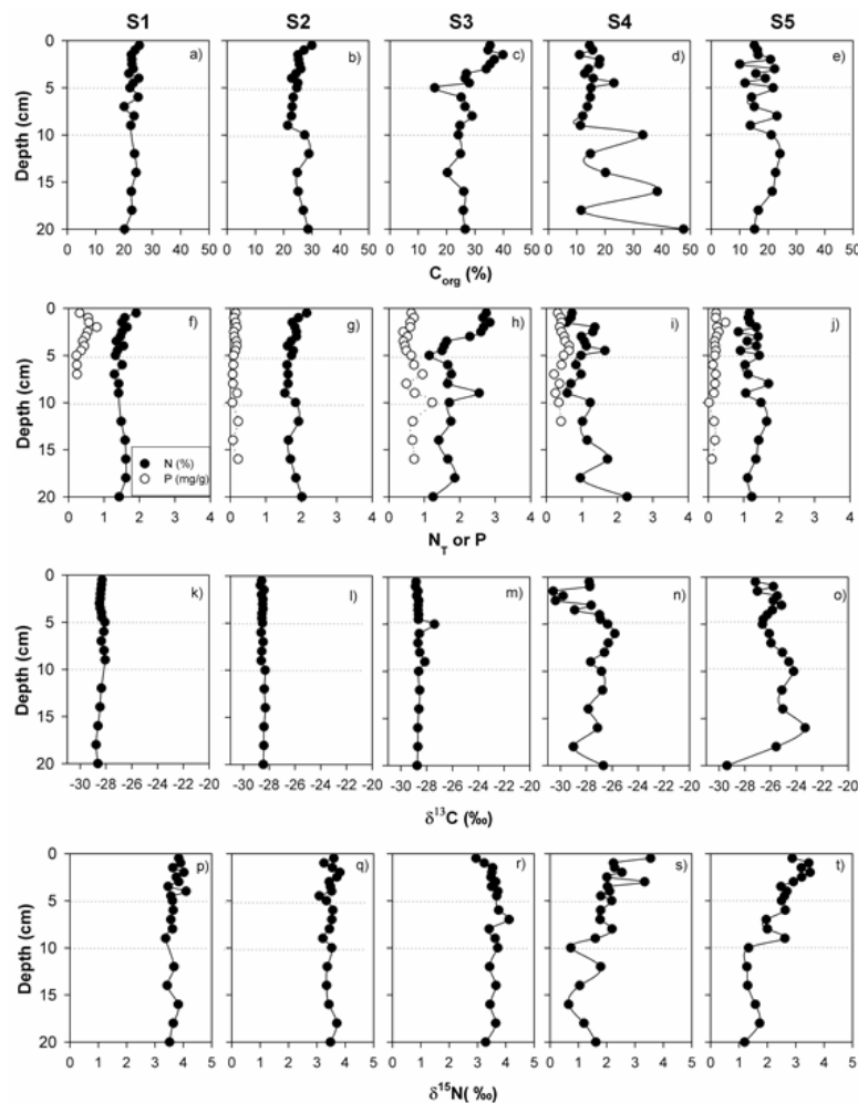
Figure 2: Vertical patterns of organic C, TN, P, \delta^{13}\text{C} , and \delta^{15}\text{N} with the depth of the sediments collected in September 2012 at sites S1-S5 in the "Ciénega Tamasopo" wetland (San Luis Potosi, Mexico).
